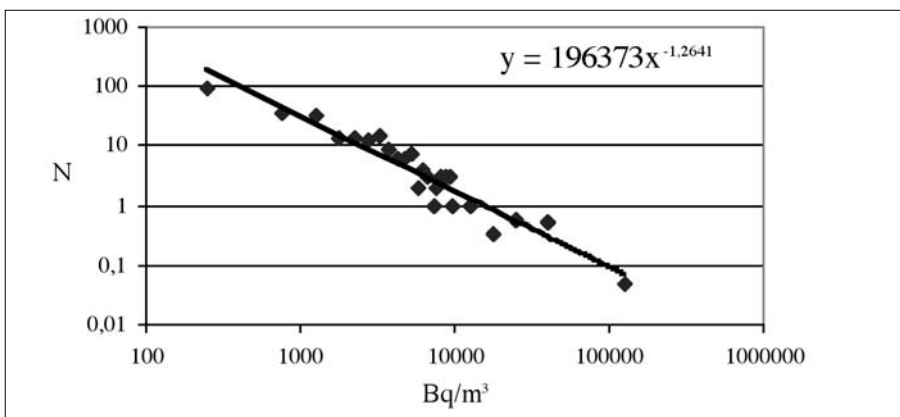
Fig. 1 - Distribution of 303 average radon concentrations from 220 caves from all over the world. Hakl (2004), within intervals of 500 Bq/m 3 .
